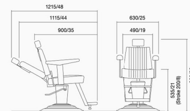
DIMENSIONS: Dainty with Slim-85 (mm/inch)
