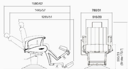
DIMENSIONS: Clipper Classic specs with Slim-R (mm/inch)
